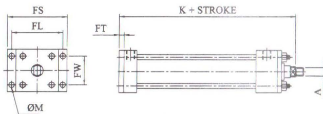
CAP END FLANGE-(BM)
