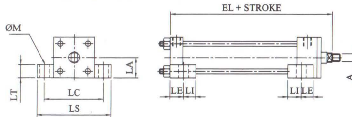
INTERMEDIATE TRUNNION-(TM)
