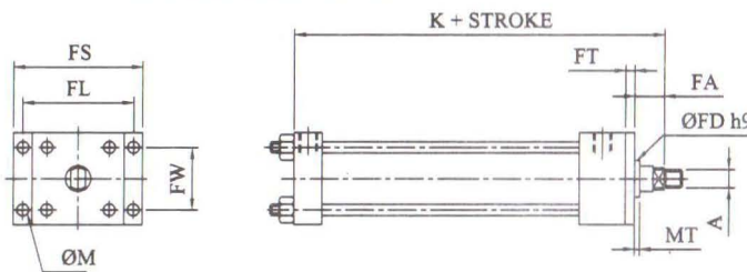
CAP END FLANGE-(BM)
